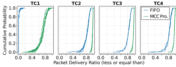
Fig. 3. Empirical distr. function of the packet delivery ratios observed in 100 runs of the bursty load scenario simulation. Every line describes the reliability of one application instance, every subplot shows one traffic class (TC).
