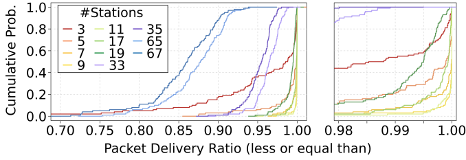
Fig. 4. Empirical distr. function of packet delivery ratios for different number of stations. Each number of stations simulated for 100 seeds. The right plot enlarges the region between 0.98 and 1.00 for better visibility.
