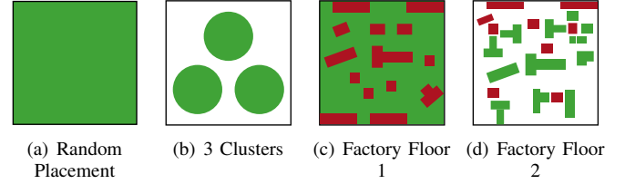
Fig. 1. Evaluation scenarios. Each has a size of 50\text{ m} \times 50\text{ m} . Green = Allowed station placement, Red = Obstacle, White = Free Space
