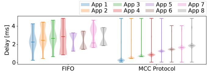
Fig. 2. Delay between packet generation and delivery observed in the burst pressure scenario for the safety-critical applications (i.e., TC1).
